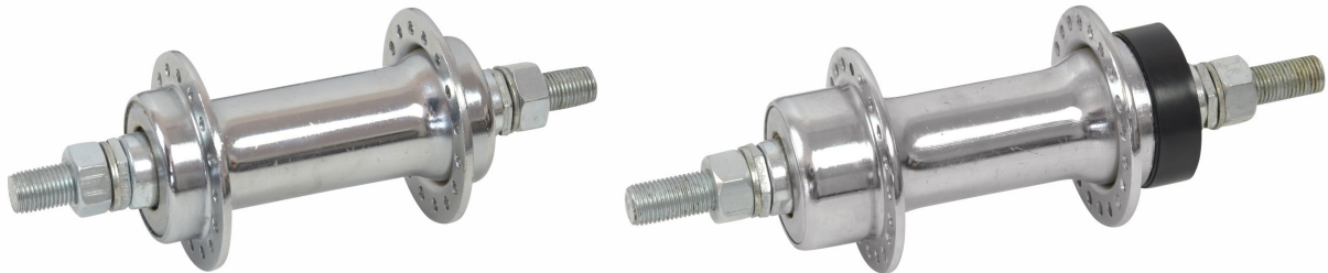
PHILLIP TYPE - HUB SET
